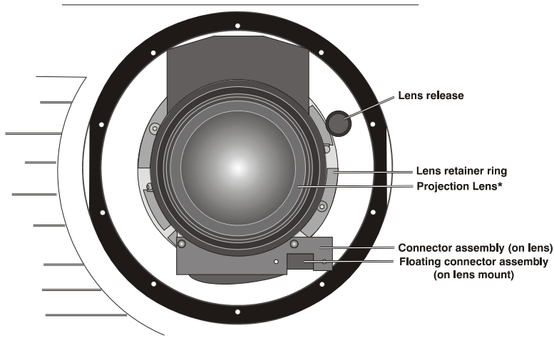
Figure 4.10. Lens Assembly
