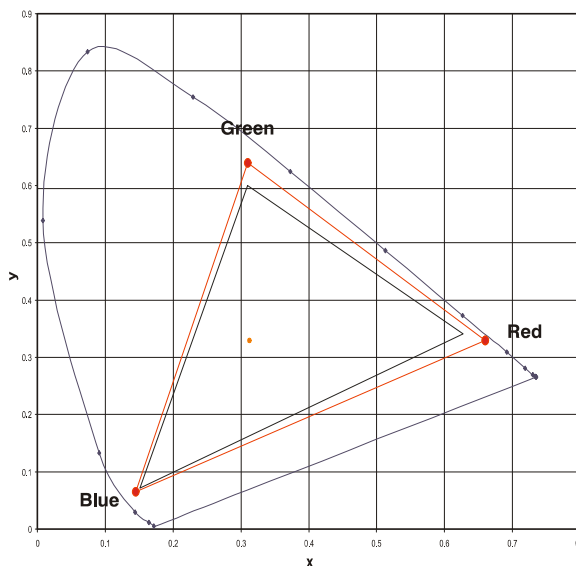
Figure 3.11. CIE 1931 Chromaticity Diagram (without Yellow Notch Filter)
